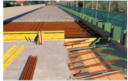
Rebar connections
